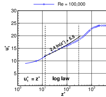
(b) u^+(z^+) distribution.
