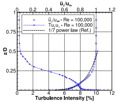
(a) Streamwise mean velocity and turbulence intensity.
