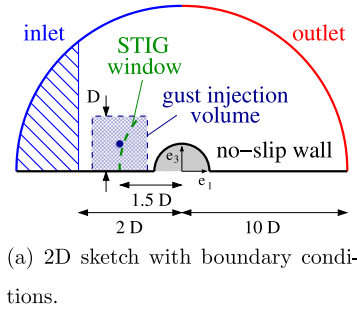
Fig. 4. Boundary conditions, STIG injection window and gust injection window used for the simulation.
