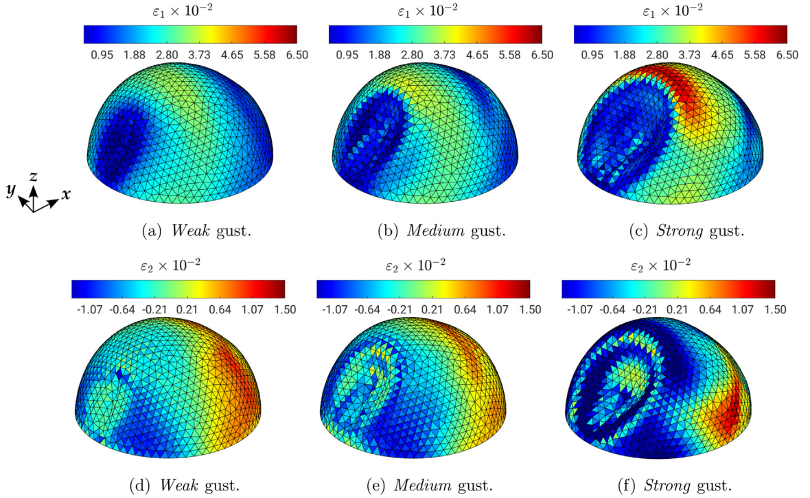
Fig. 19. Flexible FEM case: Distribution of the principal strain values \varepsilon_1 ((a) to (c)) and \varepsilon_2 ((d) to (f)) for the maximally deflected structure at different gust strengths.
